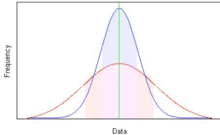
The Normal (Bell) Curve
