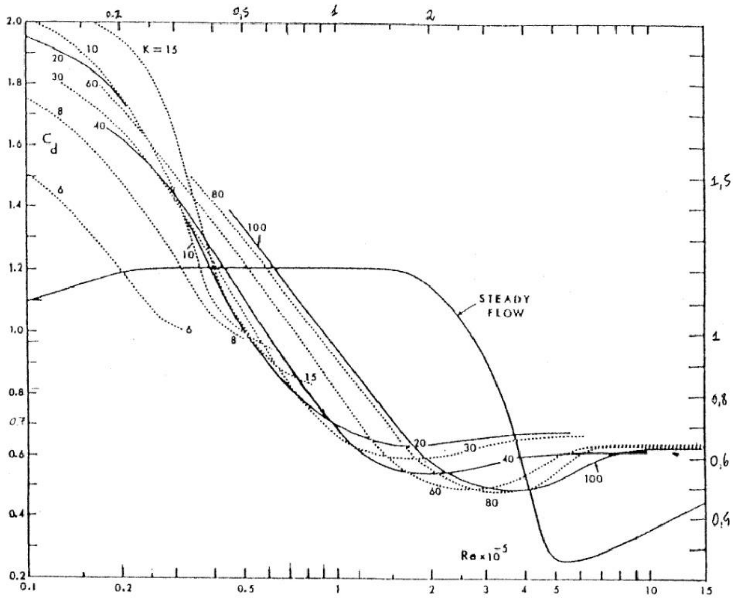
Fig. 2 – Drag coefficient versus Re for submerged cylinders (Sarpkaya & Isaacson, 1981).
