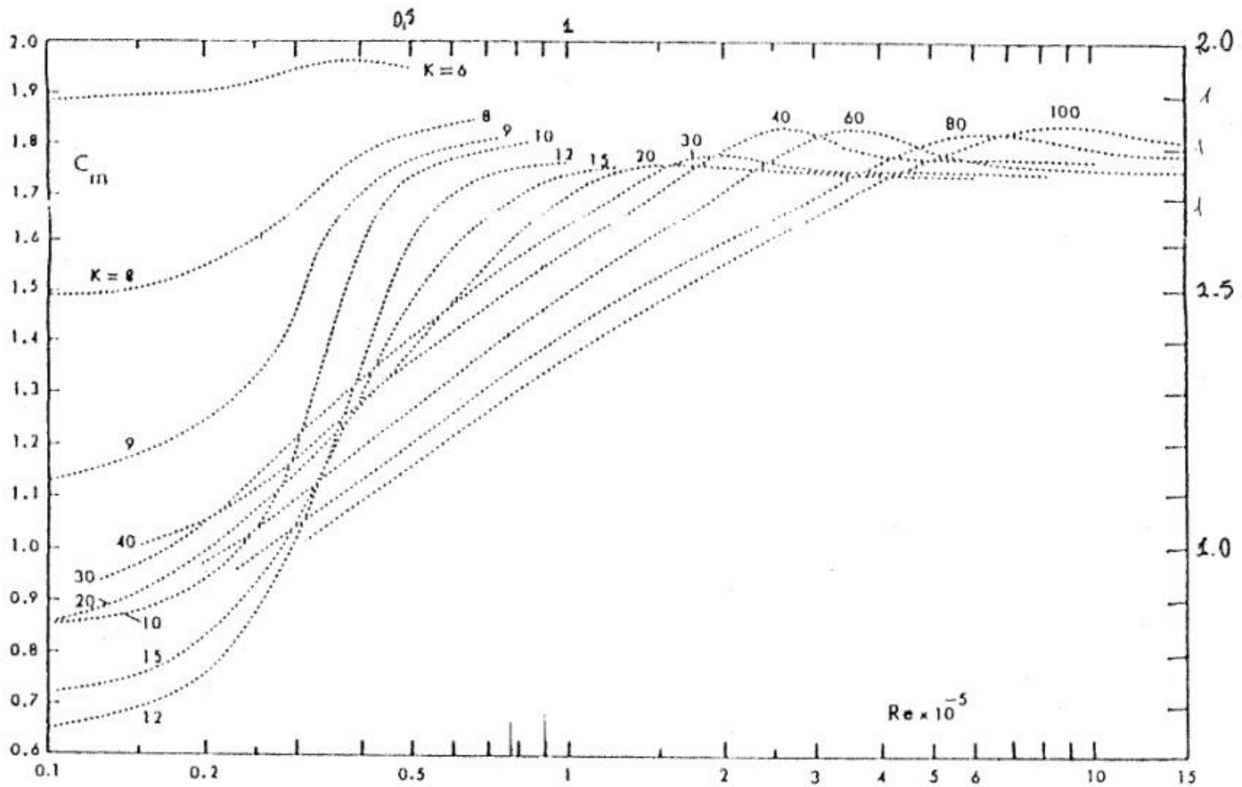
Fig. 1 – Inertia coefficient versus Re for submerged cylinders (Sarpkaya & Isaacson, 1981).
